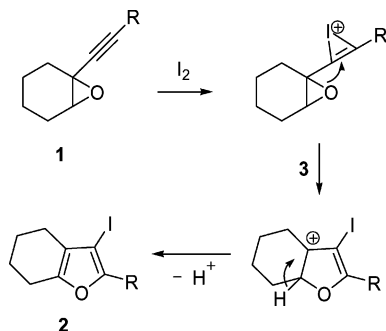
Scheme 3. Plausible reaction mechanism.
